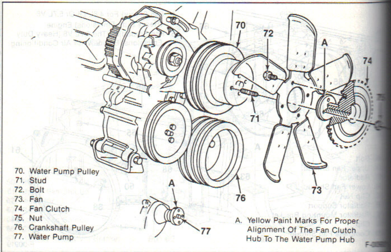
Figure 38—Fan And Fan Clutch Attachment
