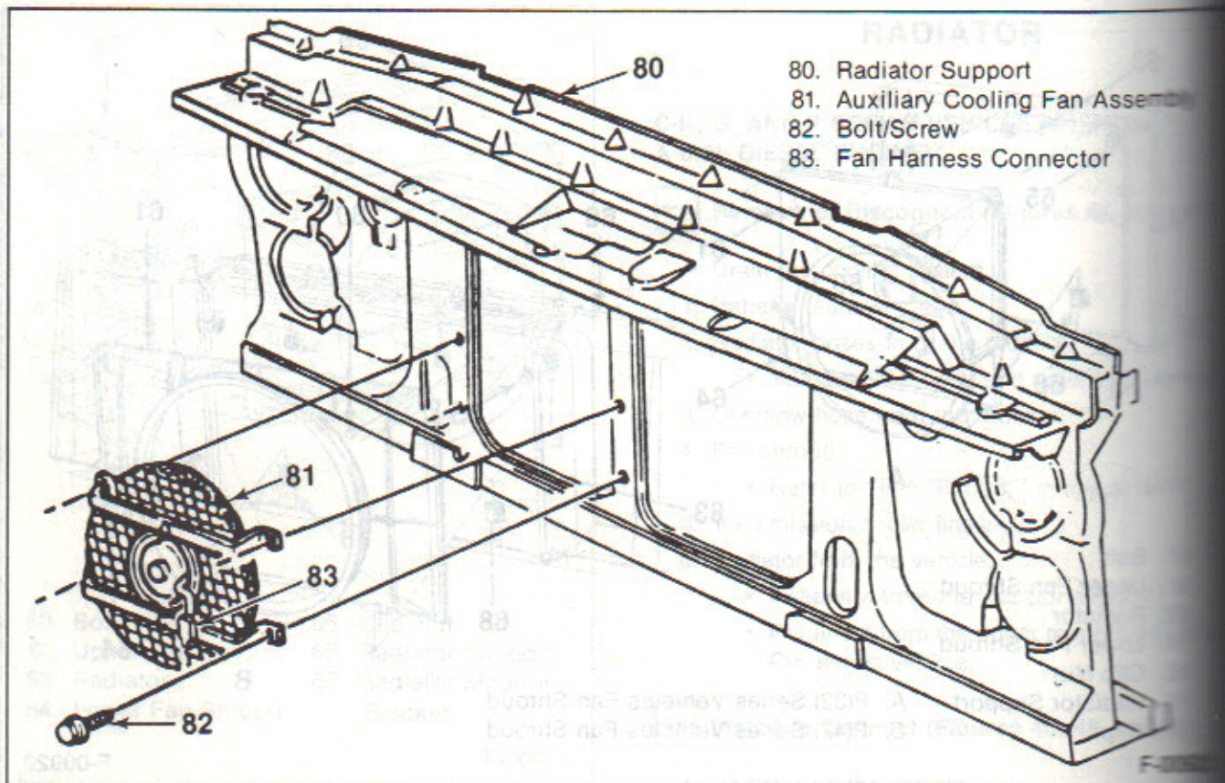
Figure 39—Auxiliary Cooling Fan Attachment
